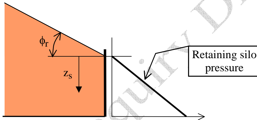
Figure 5.8: Filling pressures in retaining silo
