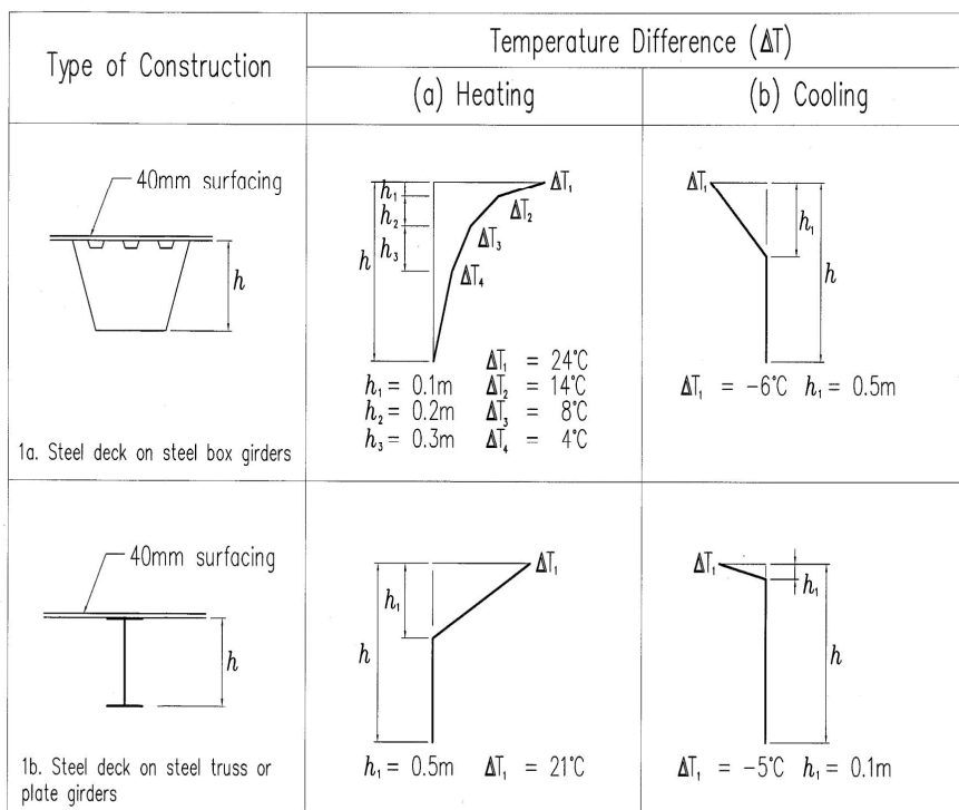
Figure 6.2a: Temperature differences for bridge decks – Type 1 : Steel Decks
