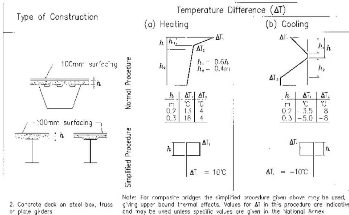
Figure 6.2b: Temperature differences for bridge decks – Type 2 : Composite Decks
